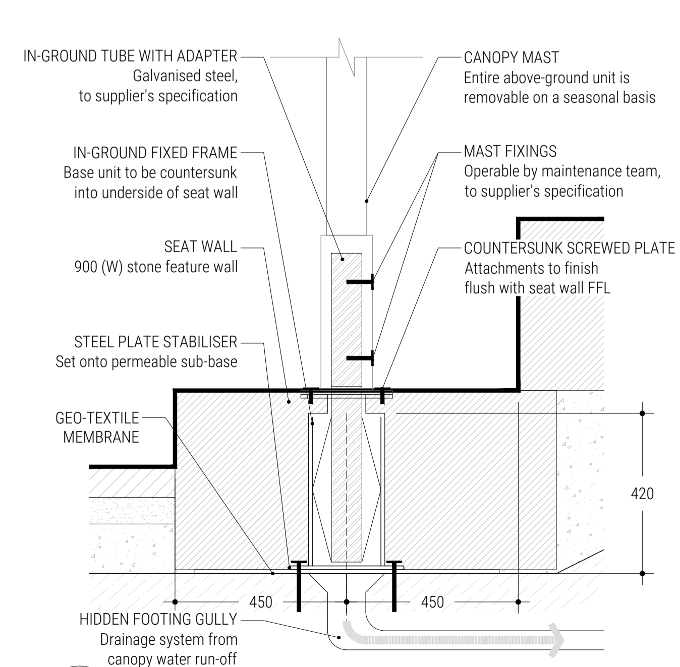
03 Section: Canopy Footing Detail L702 1:10
