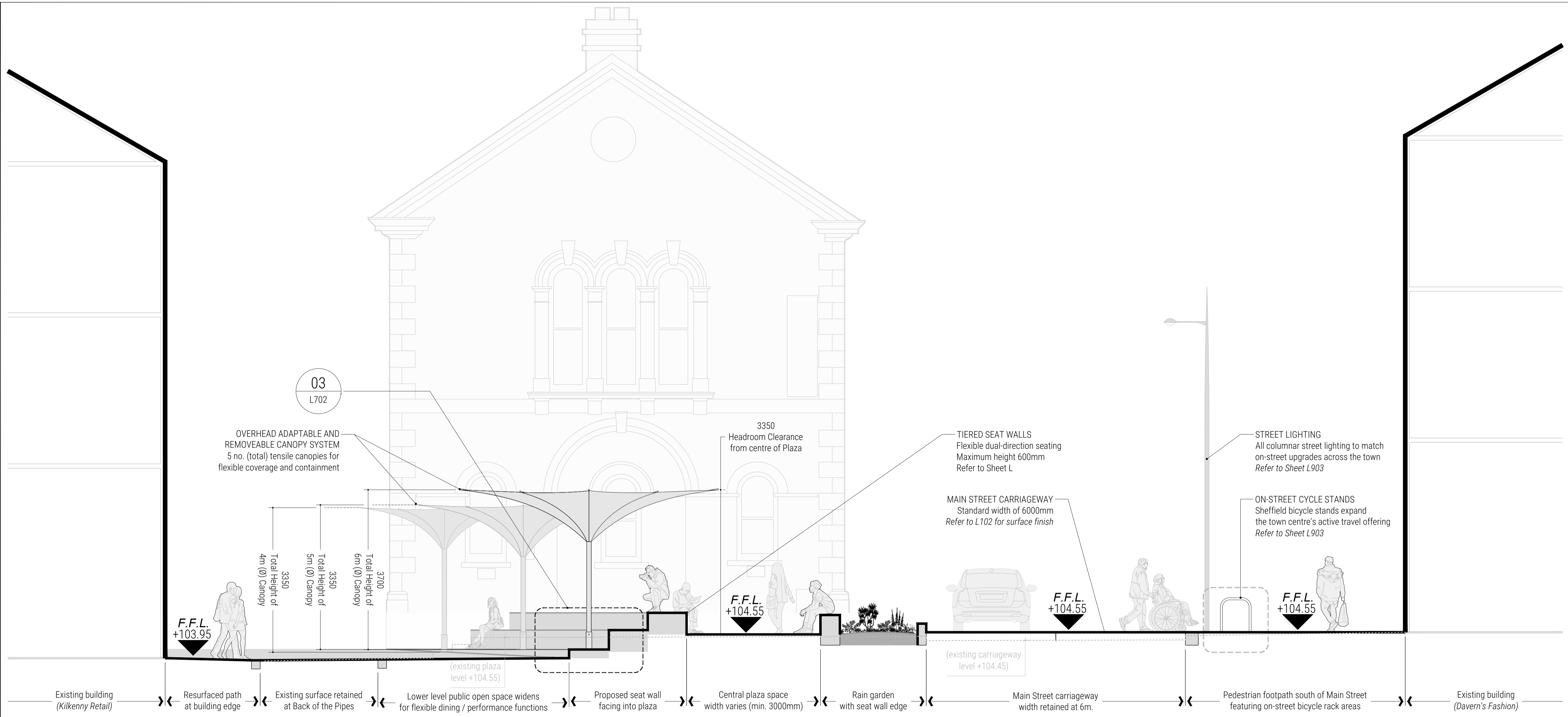
01 Section: Central Plaza Canopies L702 1:50
