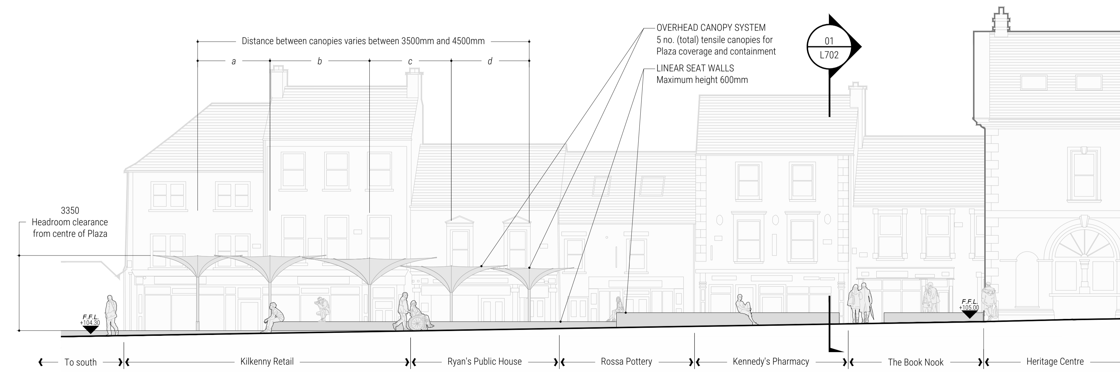
02 Elevation: Canopies (Looking North-west) L702 1:100
