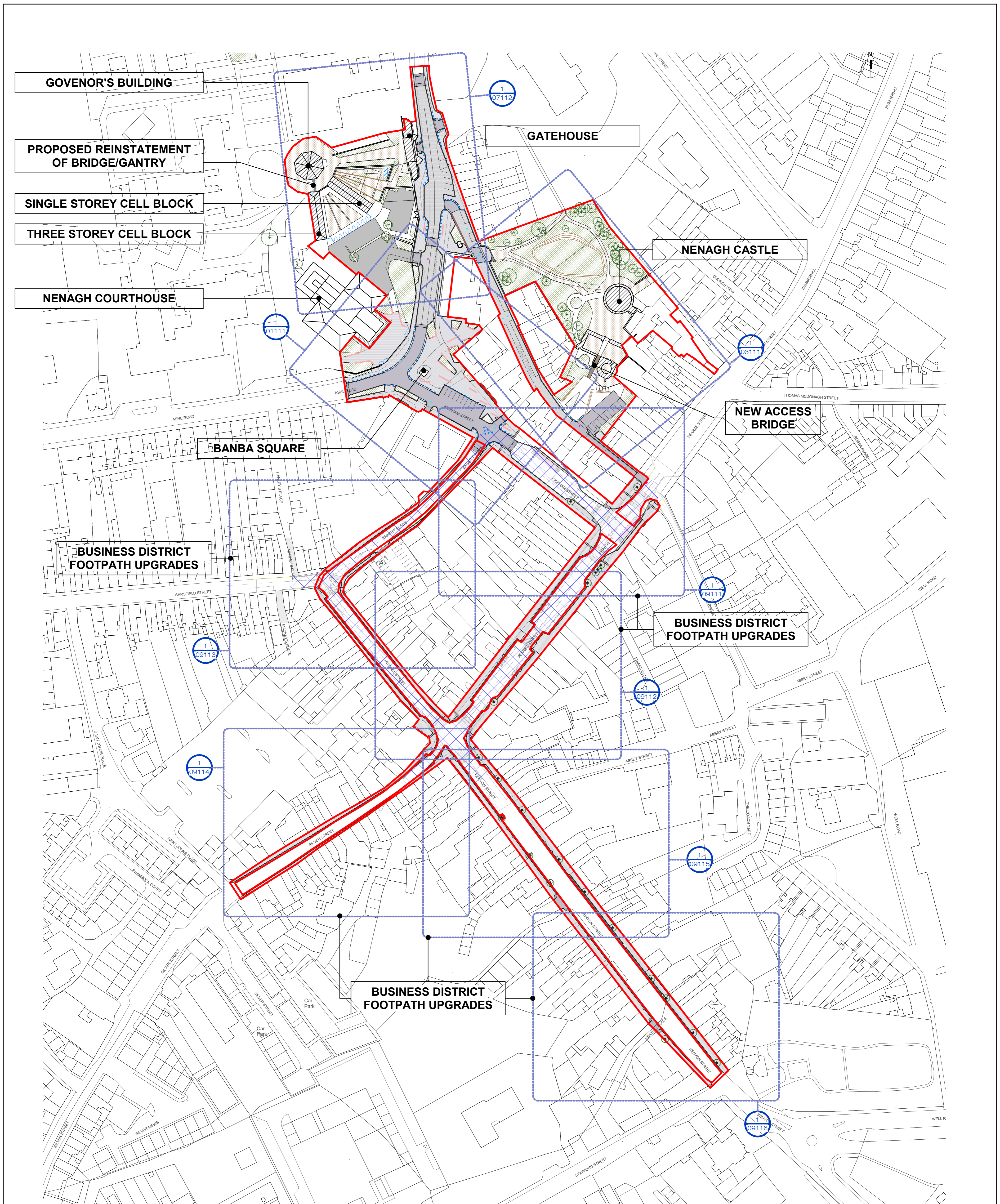
1 PROPOSED OVERALL SITE LAYOUT KEY PLAN SCALE: 1 : 1000
