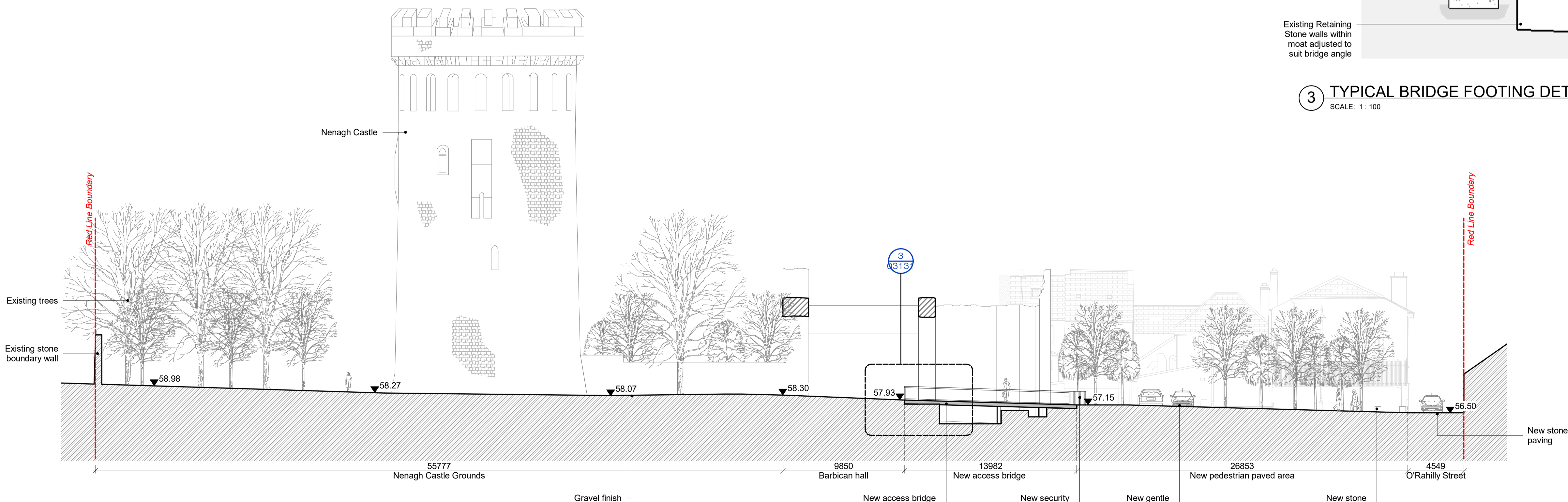
1 NENAGH CASTLE - PROPOSED SECTION SCALE: 1 : 200
