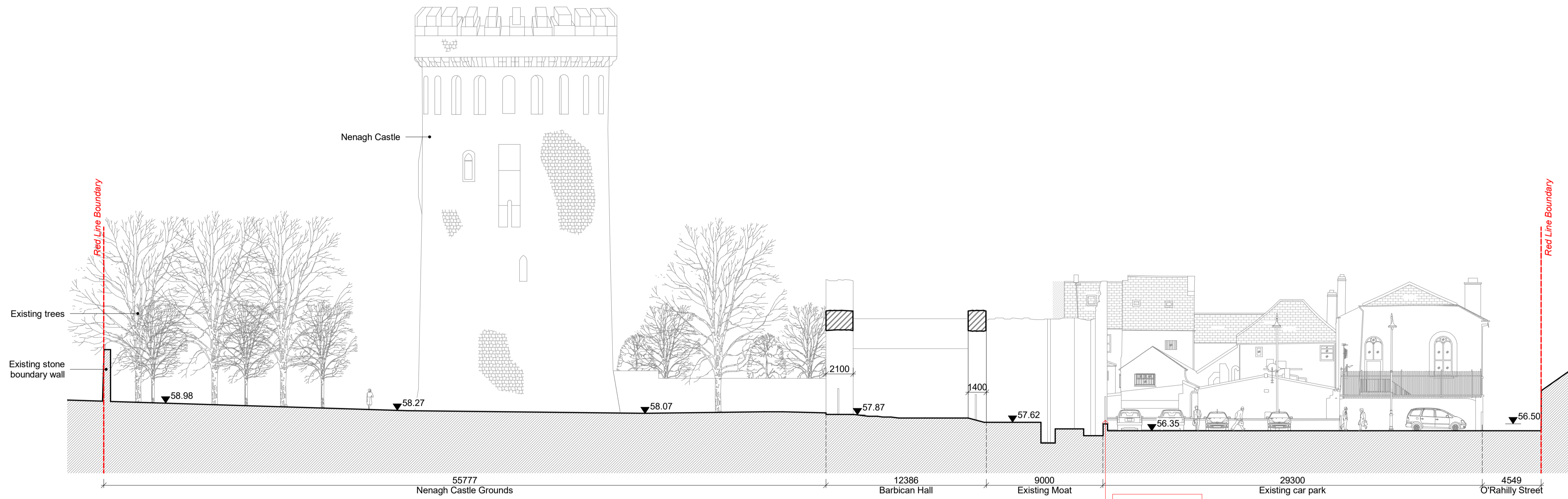
2 NENAGH CASTLE - EXISTING SECTION SCALE: 1 : 200
