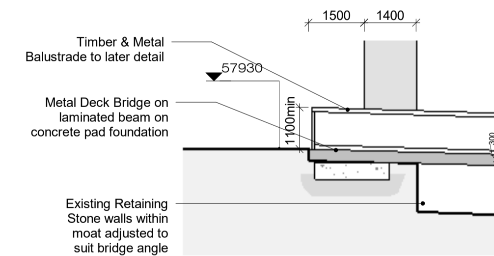
3 TYPICAL BRIDGE FOOTING DETAIL SCALE: 1 : 100
